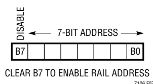
Figure 7. MFR_RAIL_ADDRESS Data Byte
