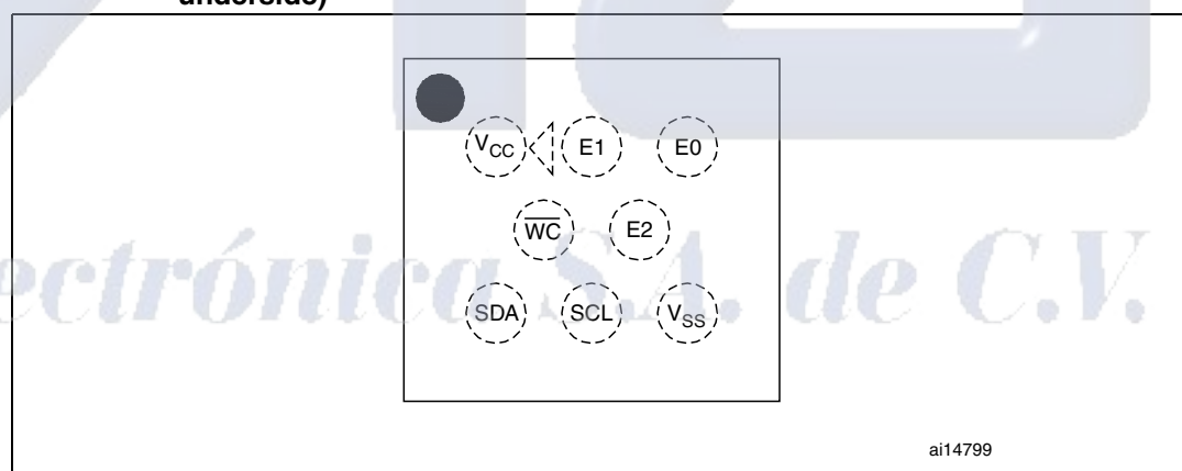
Figure 3. M24128 WLCSP connections (top view, marking side, with balls on the underside)
