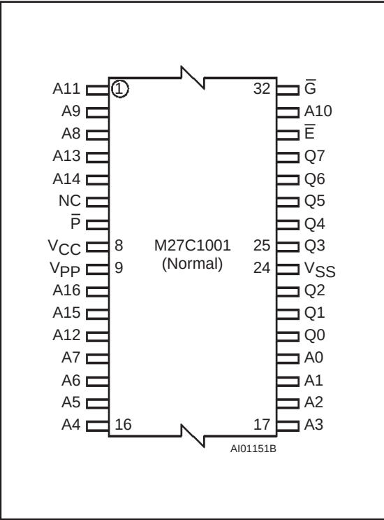
Figure 2C. TSOP Connections
