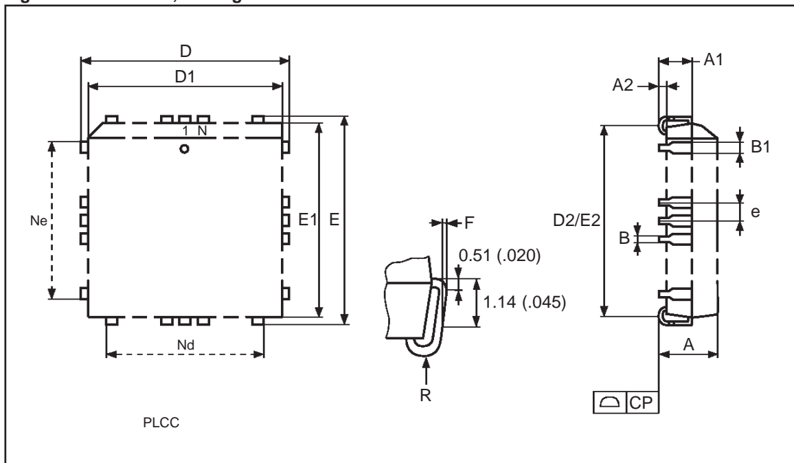
Figure 12. PLCC44 - , Package Outline
