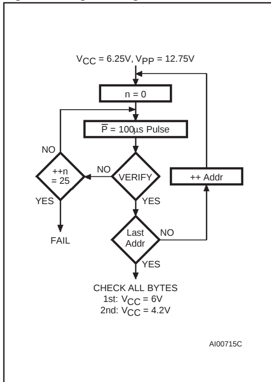
Figure 7. Programming Flowchart
