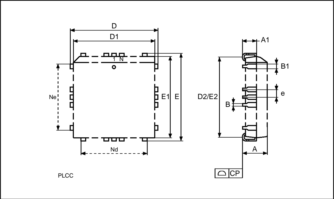
PLCC32
