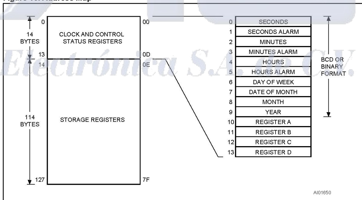
Figure 10. Address Map
