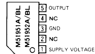
Outline 5P5T
