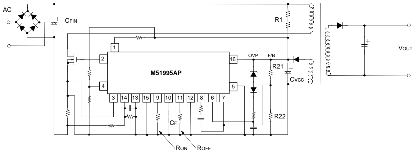
Fig.2 Example application circuit diagram of fly-back regulator
