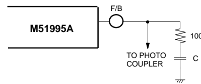
Fig.45 How to get the narrow pulse width during the start of operation
