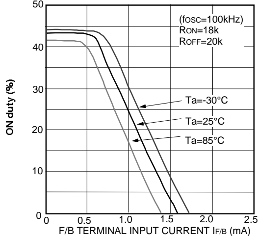
ON duty VS. F/B TERMINAL INPUT CURRENT
