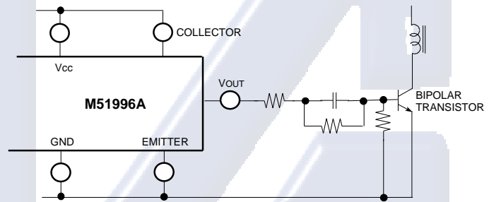
Fig.42 Driver circuit diagram (2) for bipolar transistor
