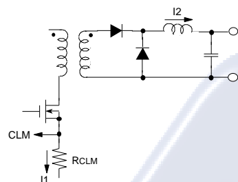
(a) Feed forward system
