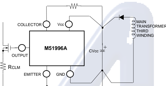
Fig.19 How to design the conductor-pattern of type M51996A on PC board (schematic example)
