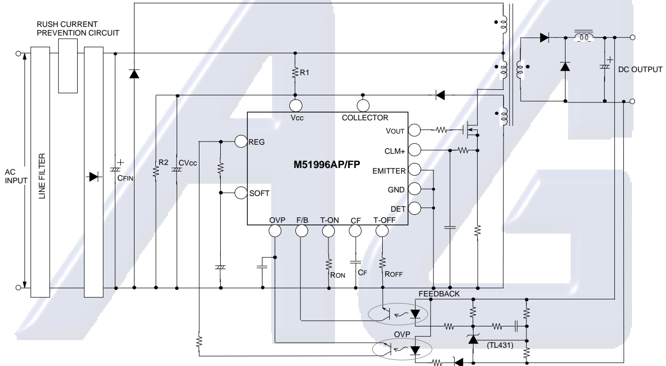
Fig.1 Application example for feed forward regulator
