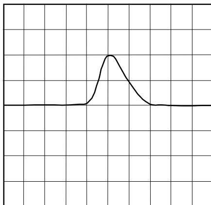
OUTPUT THROUGH CURRENT WAVEFORM AT RISING EDGE OF OUTPUT PULSE
