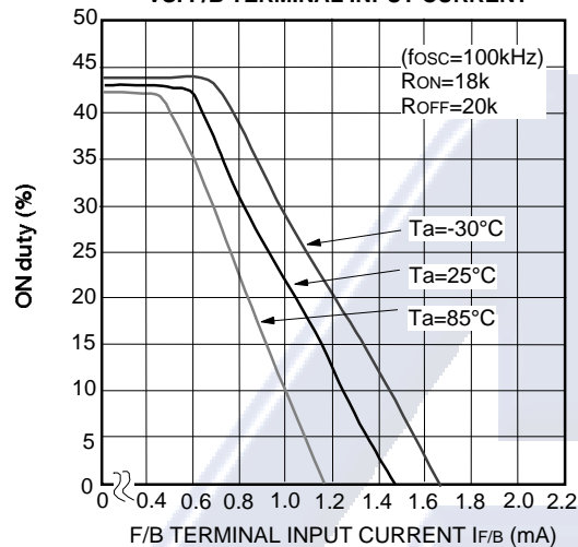
ON duty VS. F/B TERMINAL INPUT CURRENT
