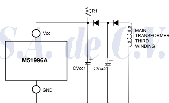
Fig.20 DC source circuit for stable start-up
