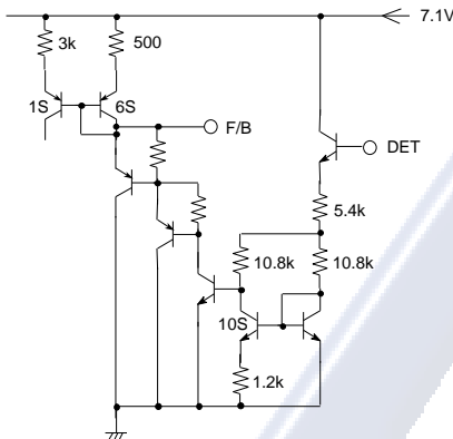
Fig.13 Voltage detector circuit section(DET)
