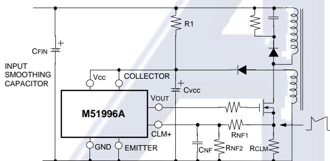
Fig.25 Peripheral circuit diagram of CLM+ terminal
