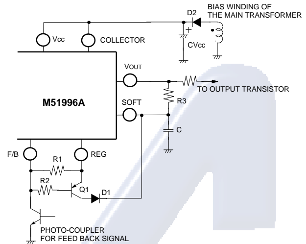
Fig.29 Current to lower frequency during over current
