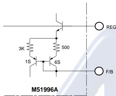
Fig.28 Relationship between REG terminal and F/B terminal
