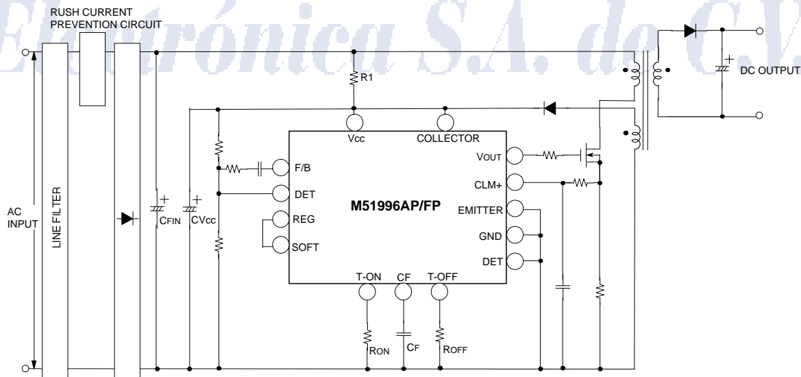
Fig.2 Application example for fly-back regulator
