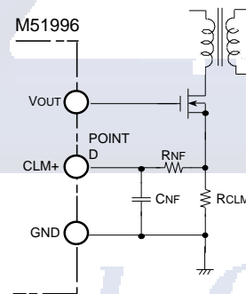
Fig.12 Connection diagram of current limit circuit
