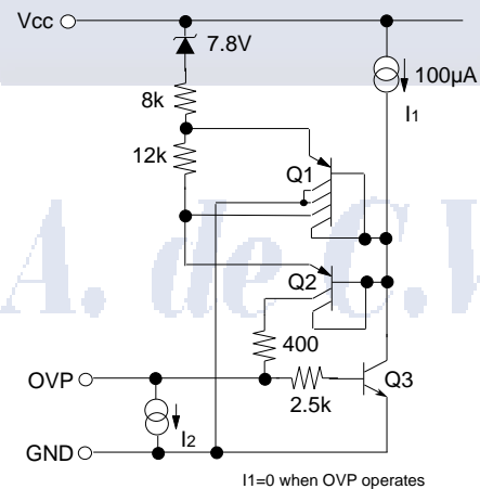
Fig.15 Detail diagram of OVP circuit
