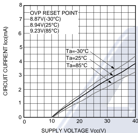
Fig.16 CIRCUIT CURRENT VS. SUPPLY VOLTAGE (OVP OPERATION)
