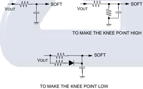
Fig.30 Method to control the knee point of frequency drop
