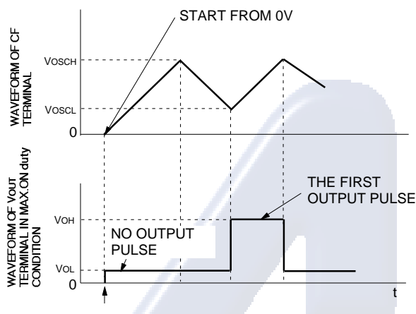
Fig.8 Relationship between oscillator waveform and output waveform at start-up
