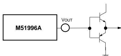
Fig.36 Output buffer circuit diagram
