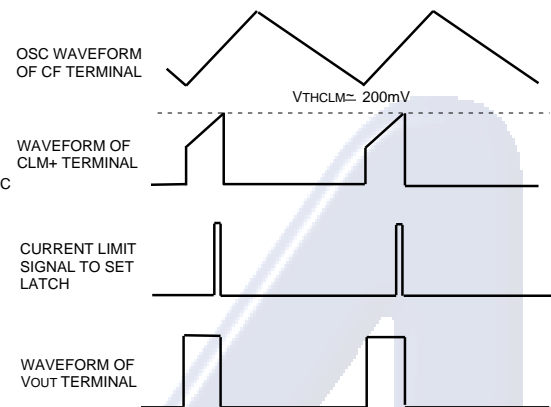
Fig.11 Operating waveform of current limiting circuit
