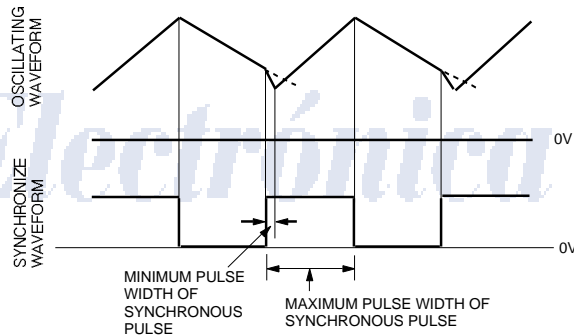
Fig.40 How to synchronize with external circuit
