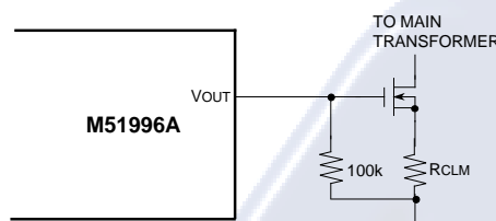
Fig.34 Circuit diagram to prevent the MOS-FET gate potential rising
