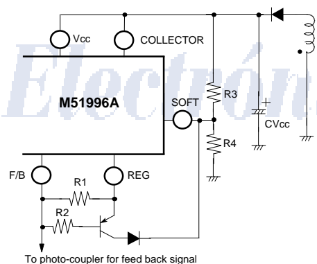
Fig.33 Current to lower the frequency during the over current in the fly back system
