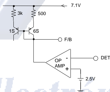
Fig.14 Schmatic diagram of voltage detector circuit section(DET)
