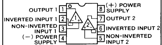
Outline 8P4 (AP) Outline 8P2S-A (AFP)
