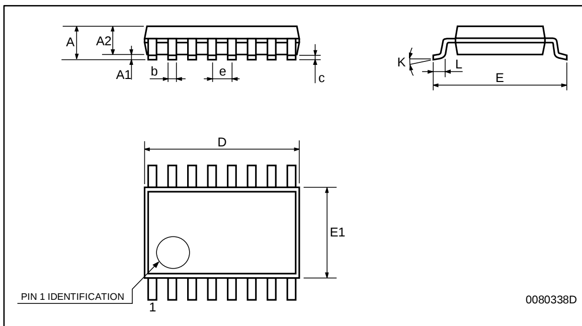
Figure 12: TSSOP16 package mechanical outline
