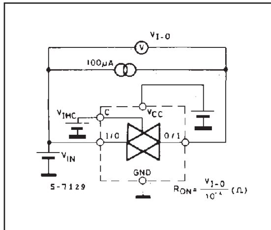
CHANNEL RESISTANCE ( R_{ON} )
