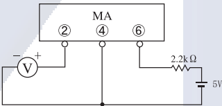
Fig1. Measurement Circuit
