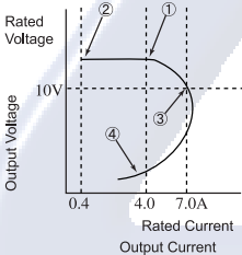
Fig2. Output Voltage/Current
