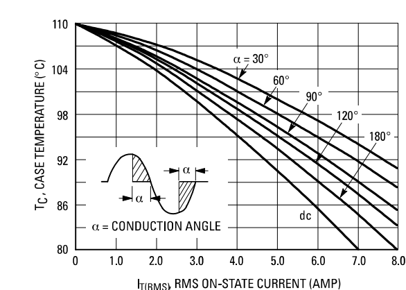
Figure 1. Current Derating
