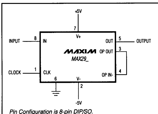
Pin Configuration is 8-pin DIP/SO.
