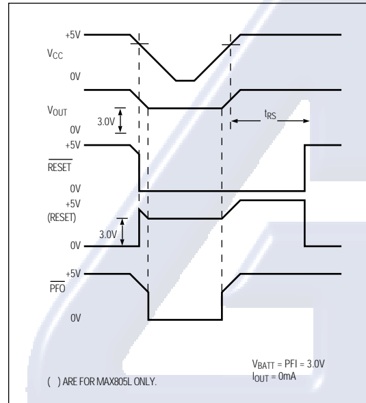
Figure 2. Timing Diagram
