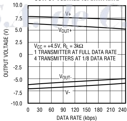
MAX205E-MAX208E OUTPUT VOLTAGE vs. DATA RATE
