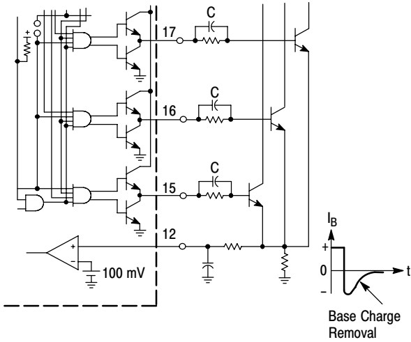
Figure 25. Current Waveform Spike Suppression
