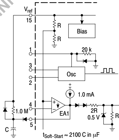
Figure 21. Soft-Start Circuit
