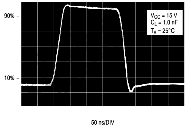
Figure 13. Output Waveform
