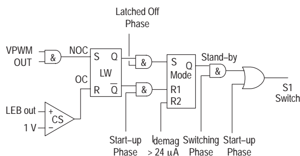
Figure 7. Transition Logic
