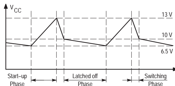
Figure 6. Hiccup Mode
