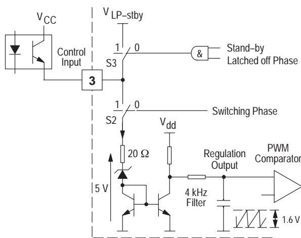
Figure 1. Regulator
