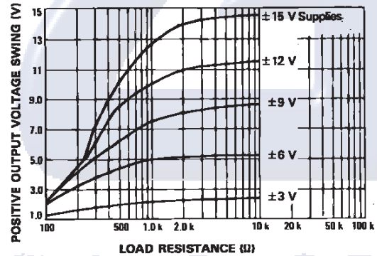
POSITIVE OUTPUT VOLTAGE SWING VERSUS LOAD RESISTANCE
