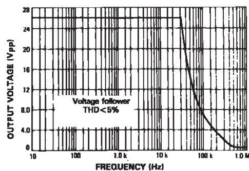
POWER BANDWIDTH (Large signal swing versus frequency)
