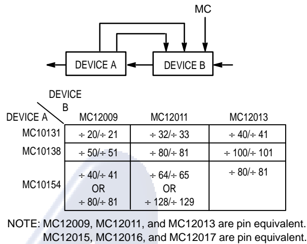
Figure 13. Dual-Modulus Values
