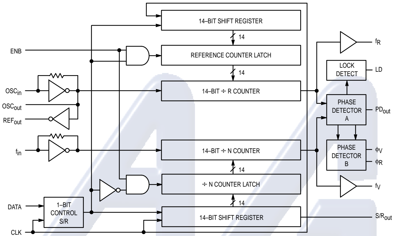
MC145157-2 BLOCK DIAGRAM
