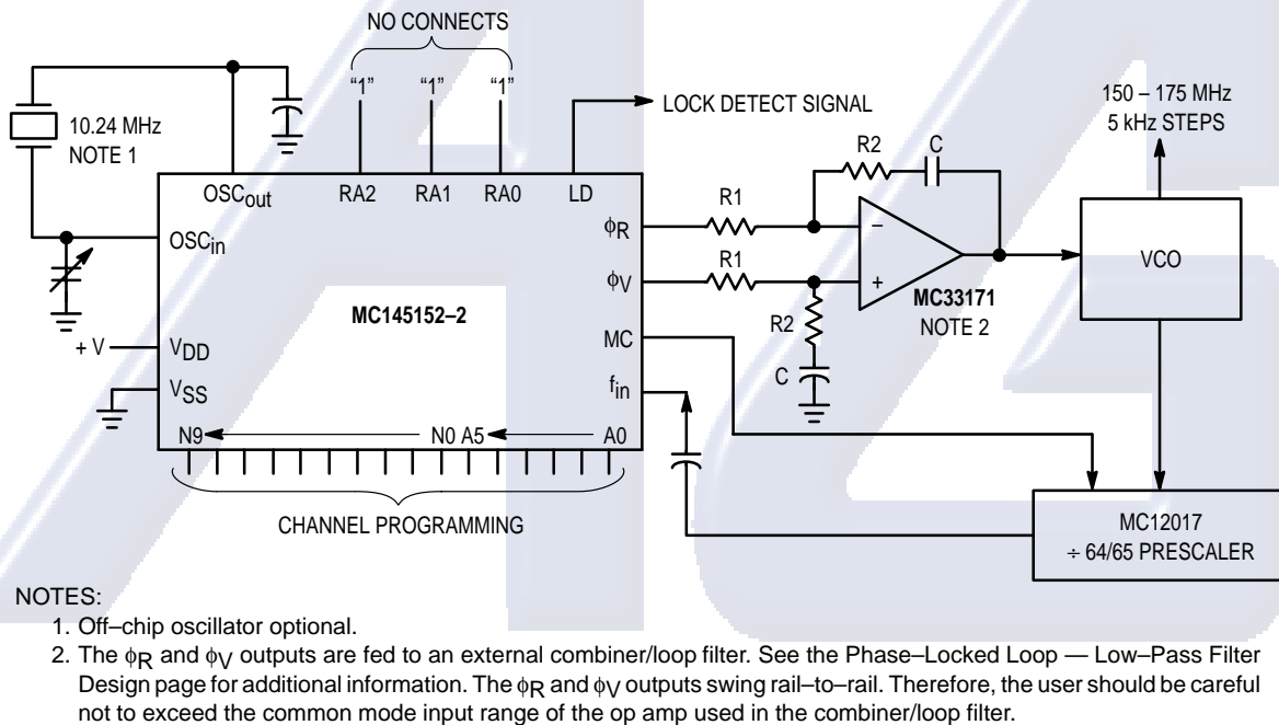
Figure 1. Synthesizer for Land Mobile Radio VHF Bands
