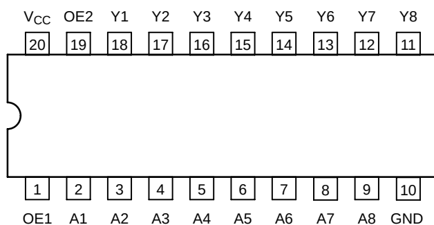
Figure 1. Pinout: 20-Lead Packages (Top View)
