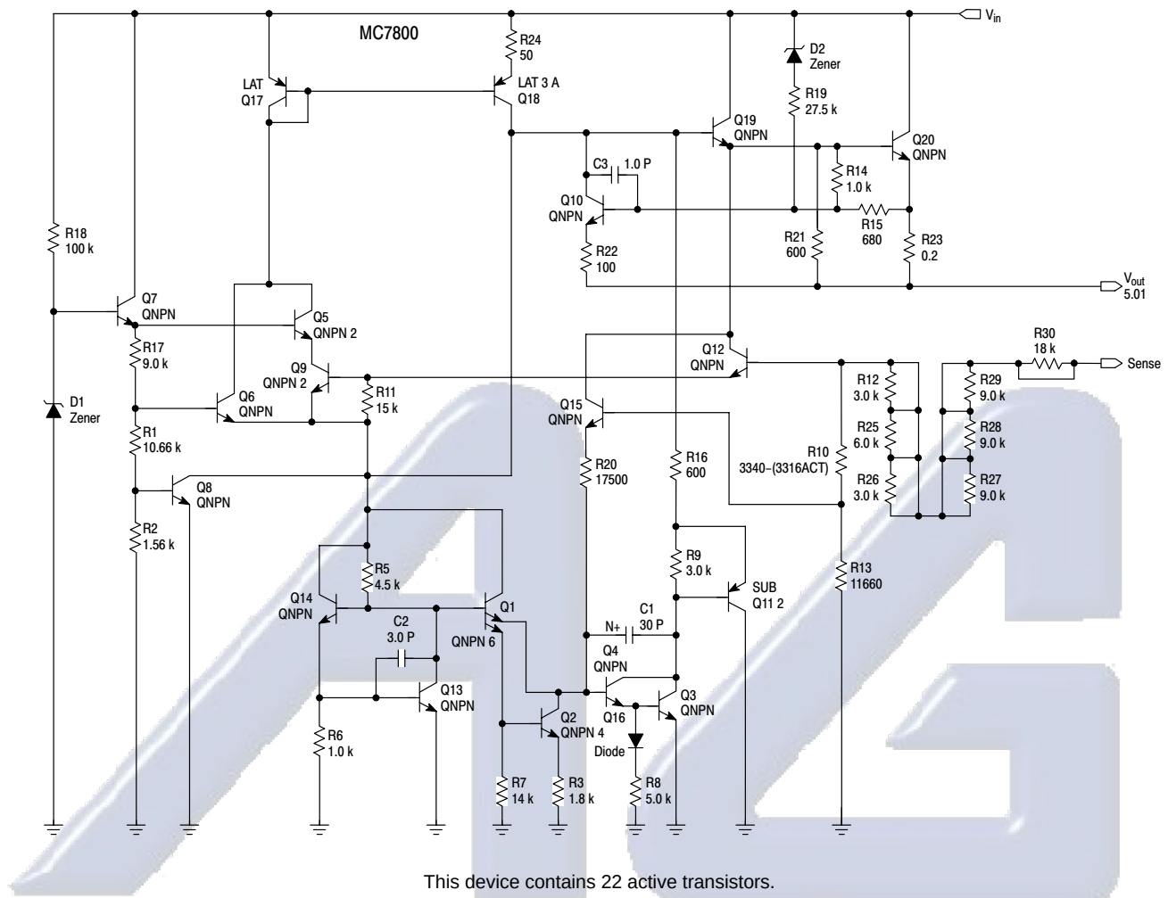
Figure 1. Representative Schematic Diagram
