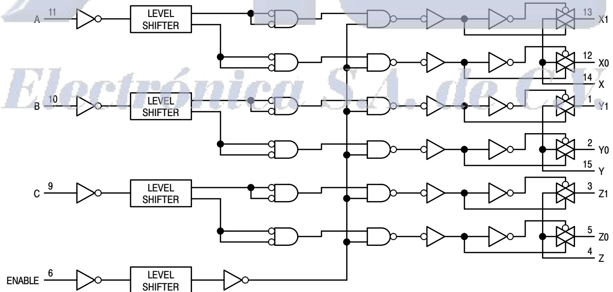
Figure 20. Function Diagram, HC4053A
