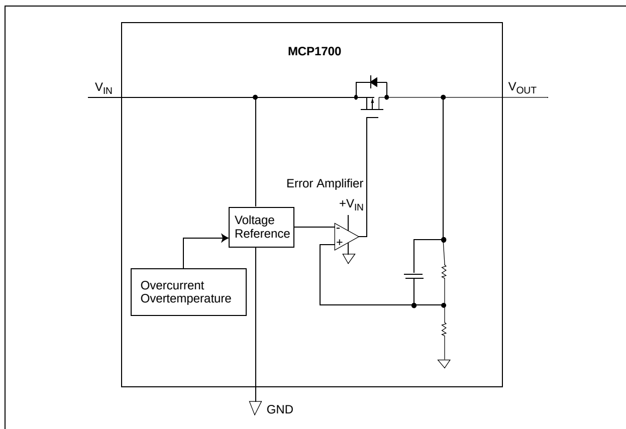
FIGURE 4-1: Block Diagram.
