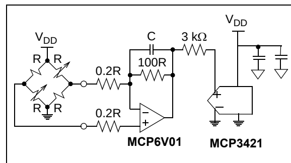
FIGURE 6-8: Simple Signal Conditioning Design with Asymmetric Circuit.
