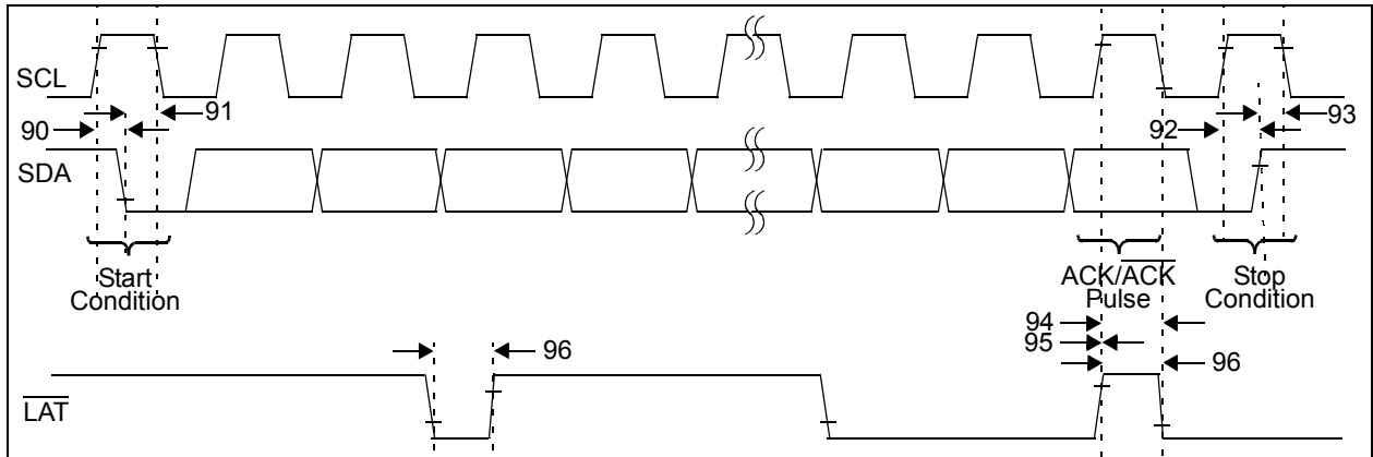
FIGURE 1-4: I 2 C™ Bus Start/Stop Bits Timing Waveforms.
