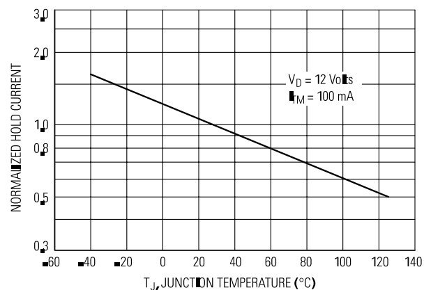
Figure 8. Holding Current
