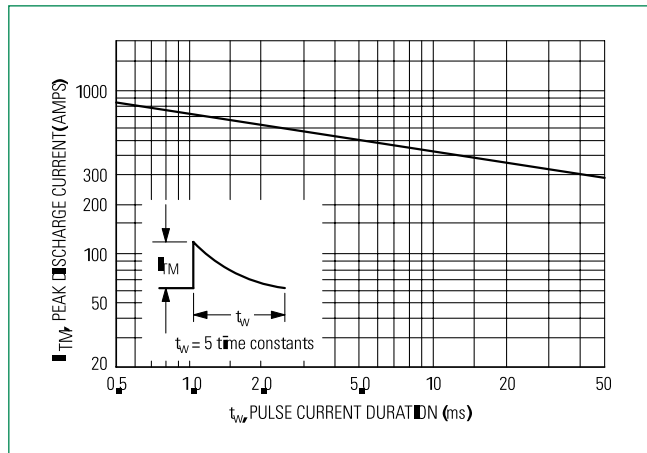
Figure 3. Current Derating
