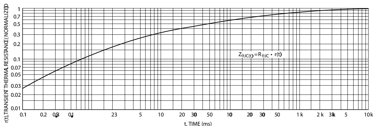
Figure 5. Thermal Response
