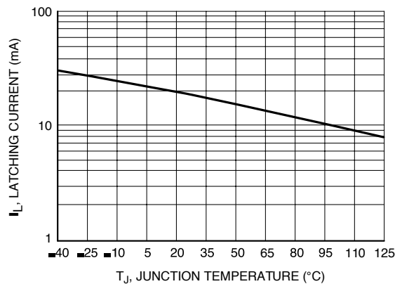
Figure 7. Typical Latching Current vs Junction Temperature
