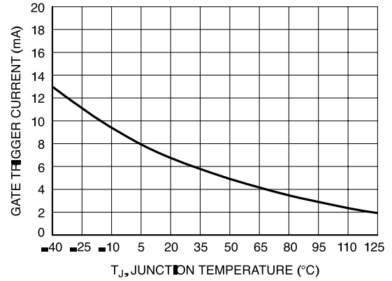
Figure 4. Typical Gate Trigger Current vs Junction Temperature
