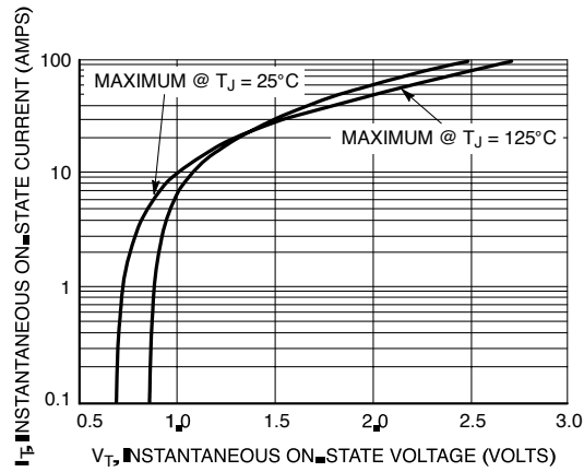
Figure 3. Typical On-State Characteristics
