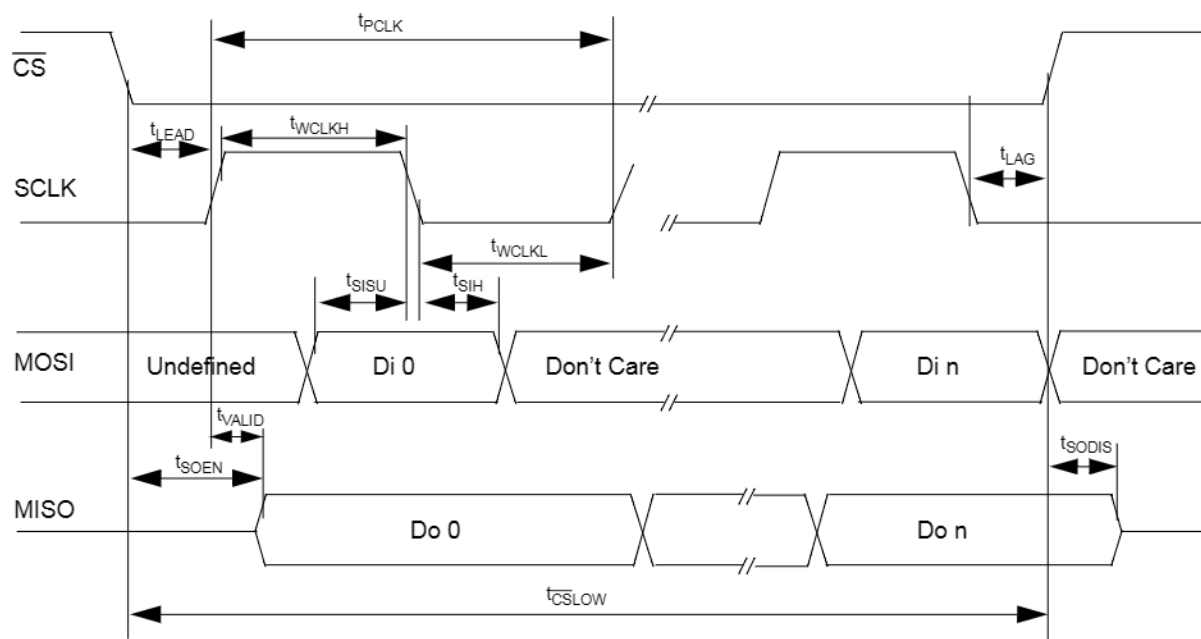
Figure 14. SPI Timings
