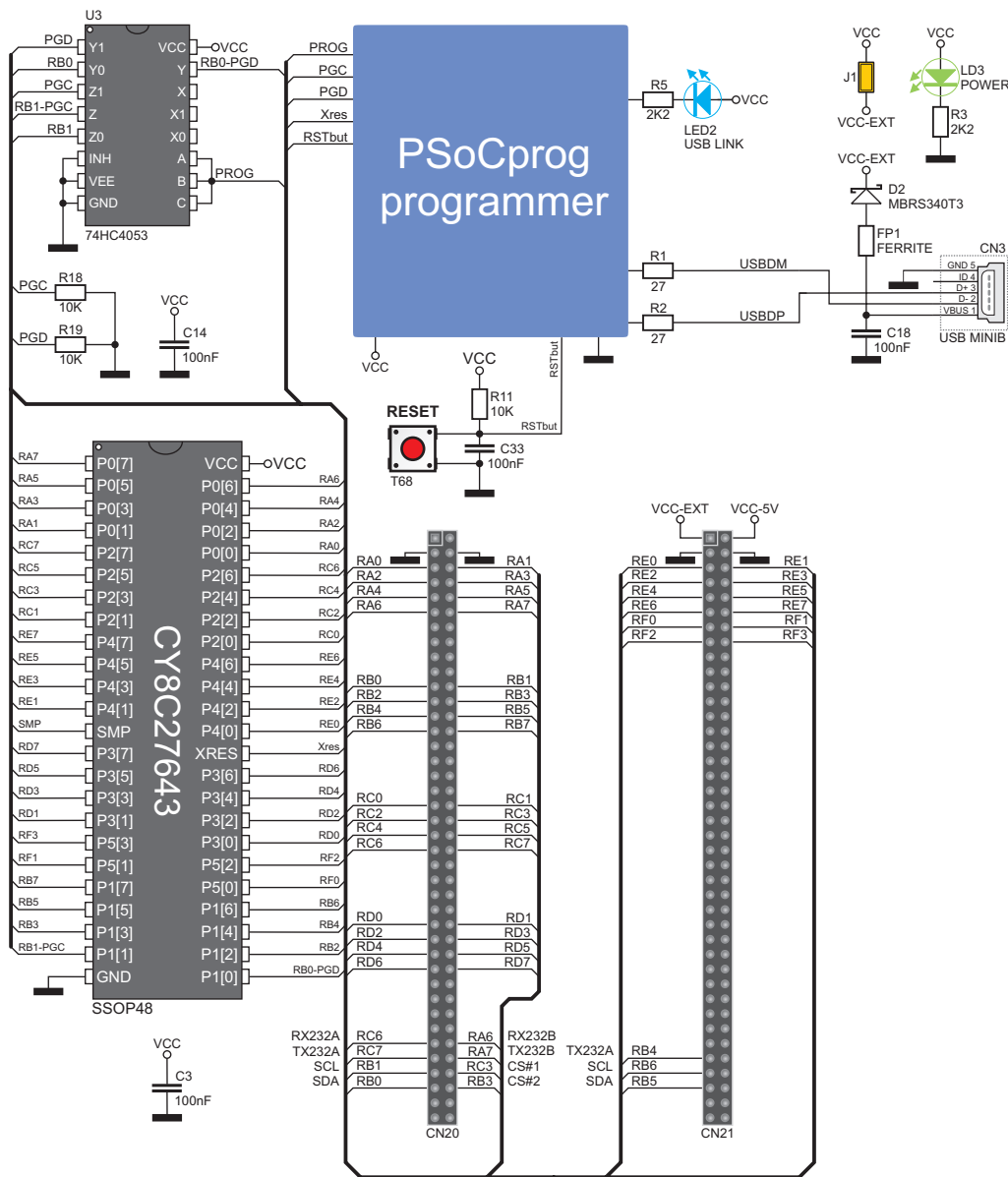
Figure 2: Connection schematic for mikroBoard
