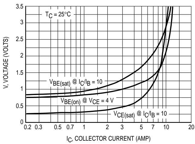
Figure 4. "On" Voltages
