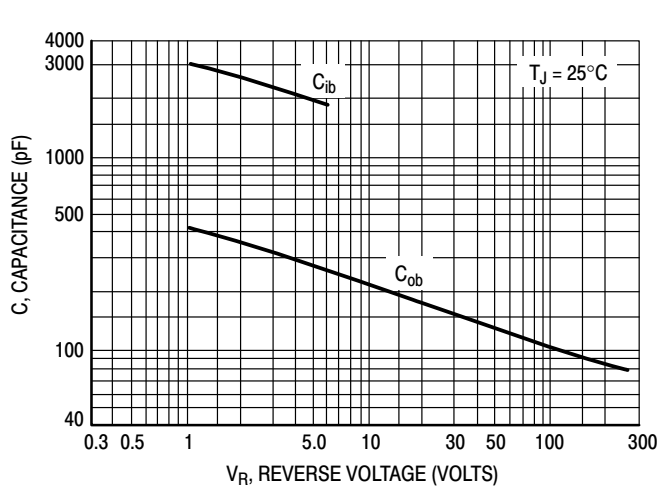
Figure 2. Capacitances
