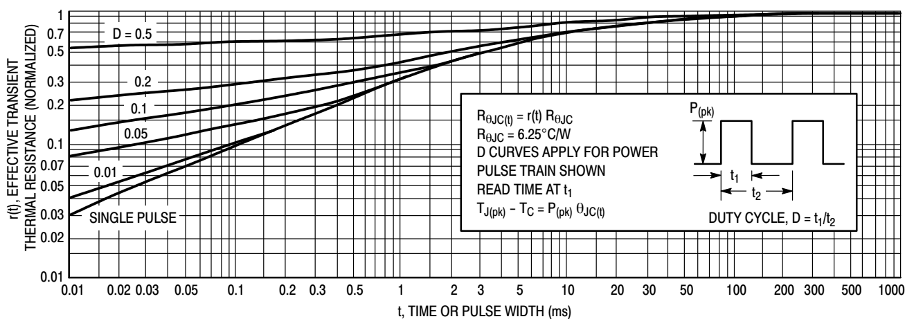
Figure 3. Thermal Response
