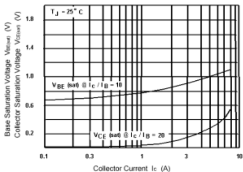
Fig.5 Base-Emitter Saturation Voltage Collector-Emmitter Saturation Voltage
