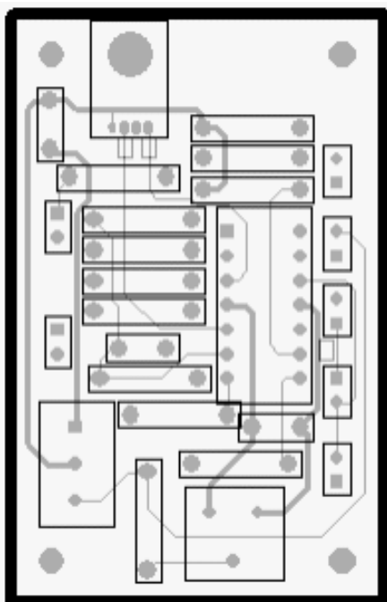
Back Side
