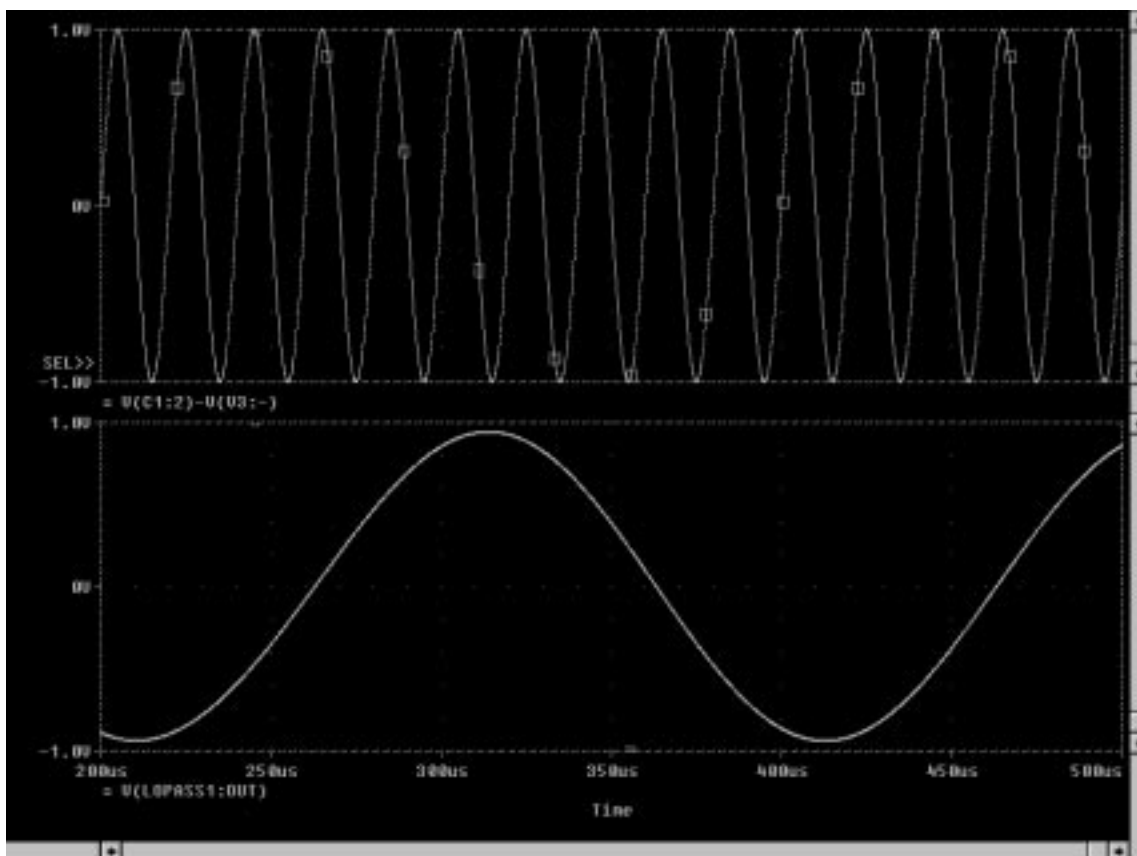
Figure 1. Aliased Signals
