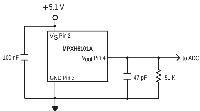
Figure 3. Recommended power supply decoupling and output filtering.
