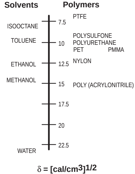
Figure 6. Typical values of solubility parameter ( \delta [cal/cm 3 ] 1/2 ) for solvents and polymers.
