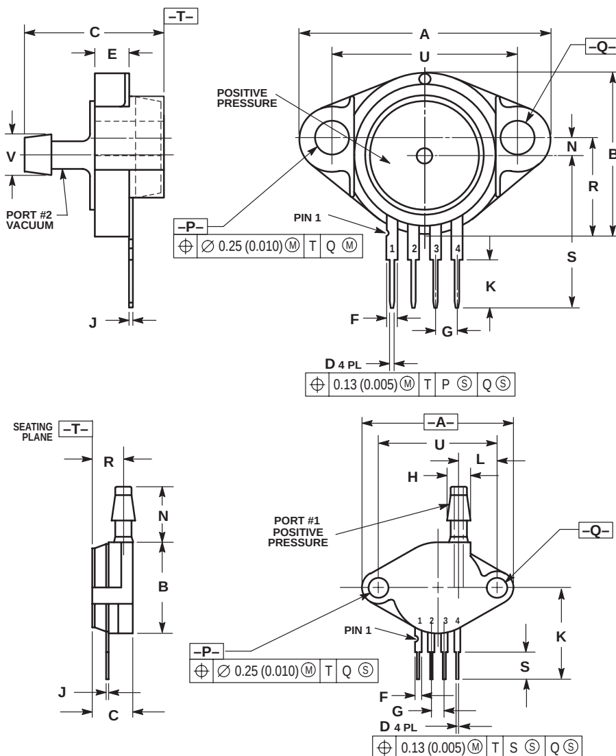
Figure 3. Case Outline Drawings
