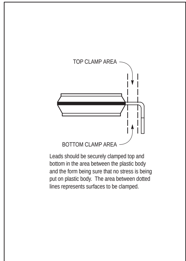
Figure 7. Leadforming
