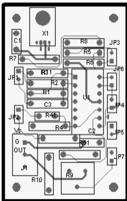
Component Side
