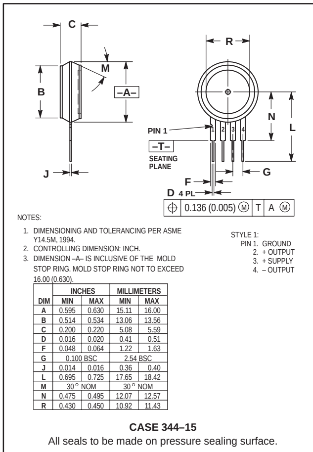
Figure 6. Chip-Carrier Package
