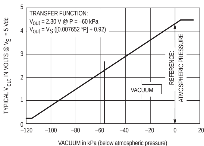
Figure 6. MPXV6115VC6U Transfer Function
