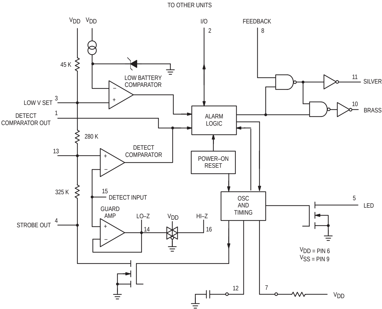
Figure 1. Block Diagram
