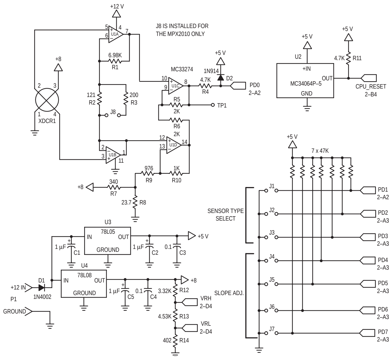
Figure 3a. Schematic
