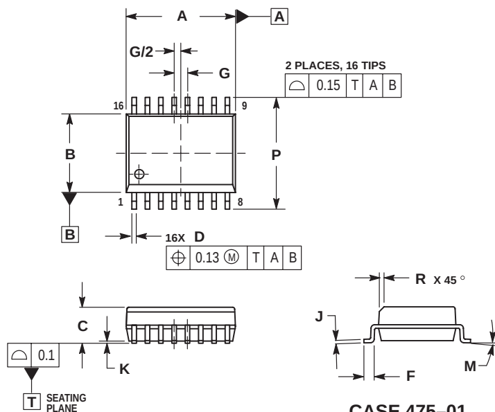
CASE 475-01 ISSUE B 16 LEAD SOIC
