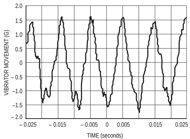
Figure 5. Vibrator Waveform
