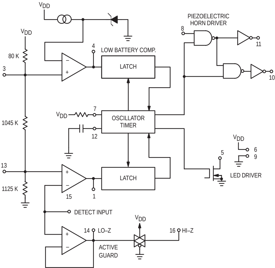
Figure 1. Block Diagram
