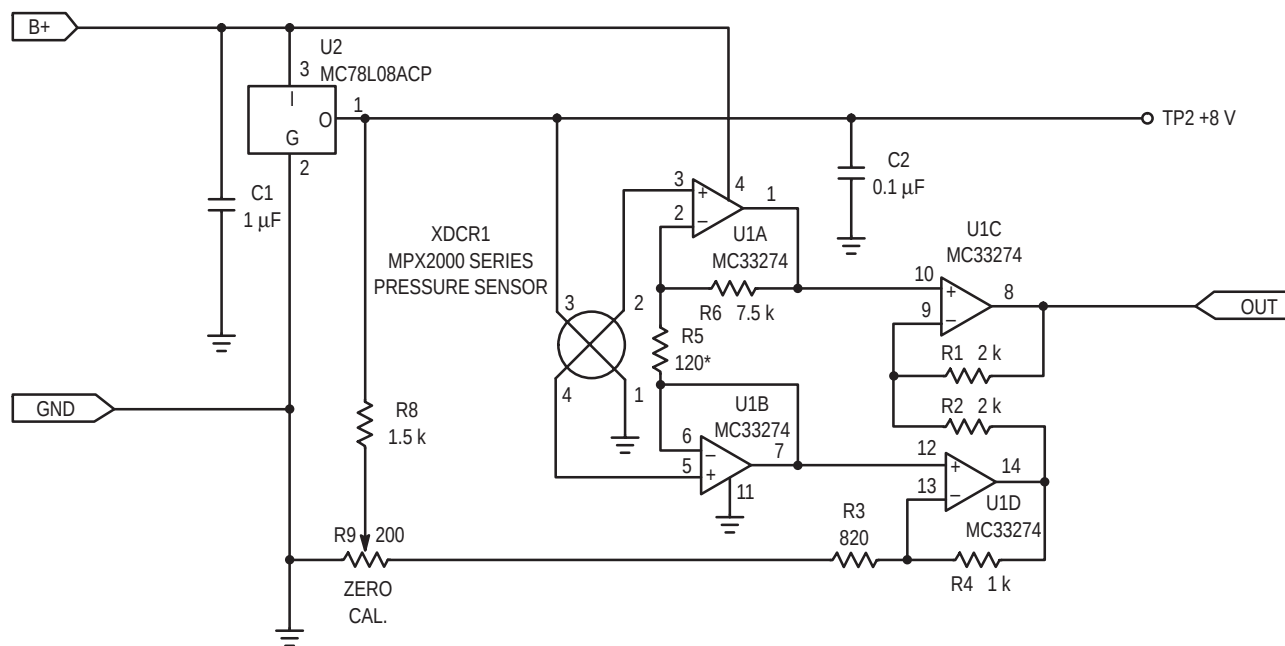
Figure 3. Sensor Specific Amplifier
