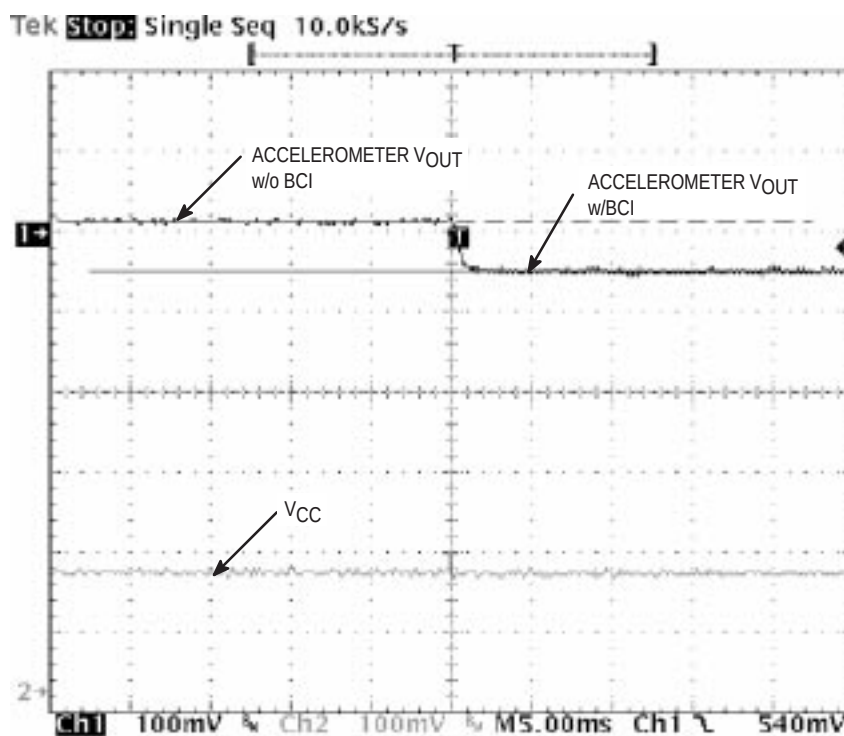
Figure 2. Accelerometer Tested Under High Frequency BCI
