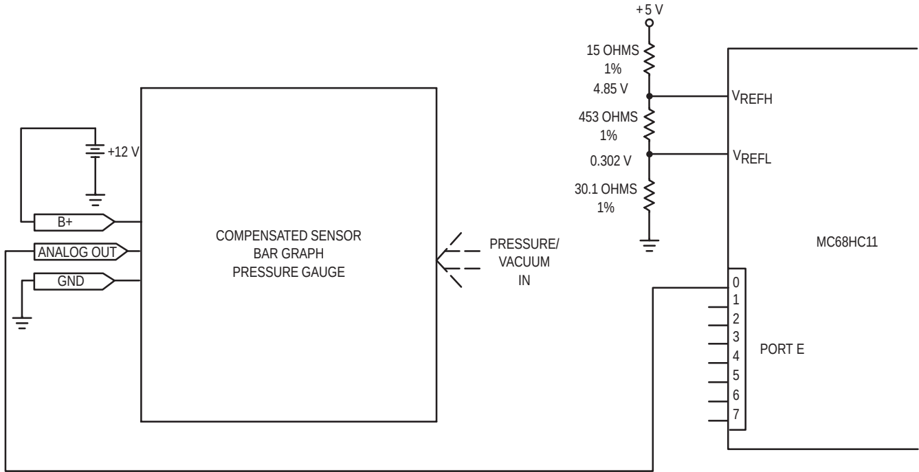
Figure 5. Application Example
