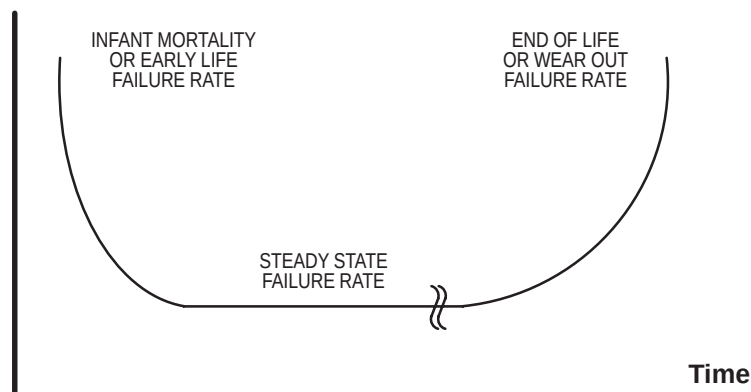
Figure 14. Bathtub curve showing various failure rate regions.
