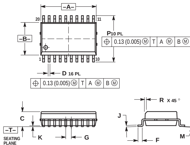
CASE 475A-01 ISSUE O 20 LEAD SOIC
