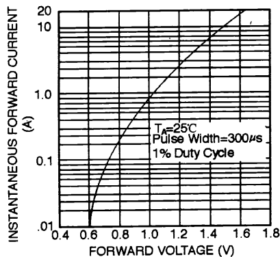
FIG. 3 – TYPICAL FORWARD CHARACTERISTICS
