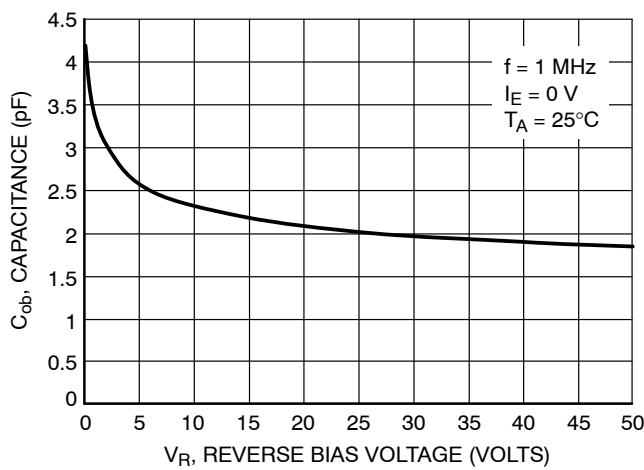
Figure 59. Output Capacitance
