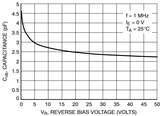
Figure 64. Output Capacitance
