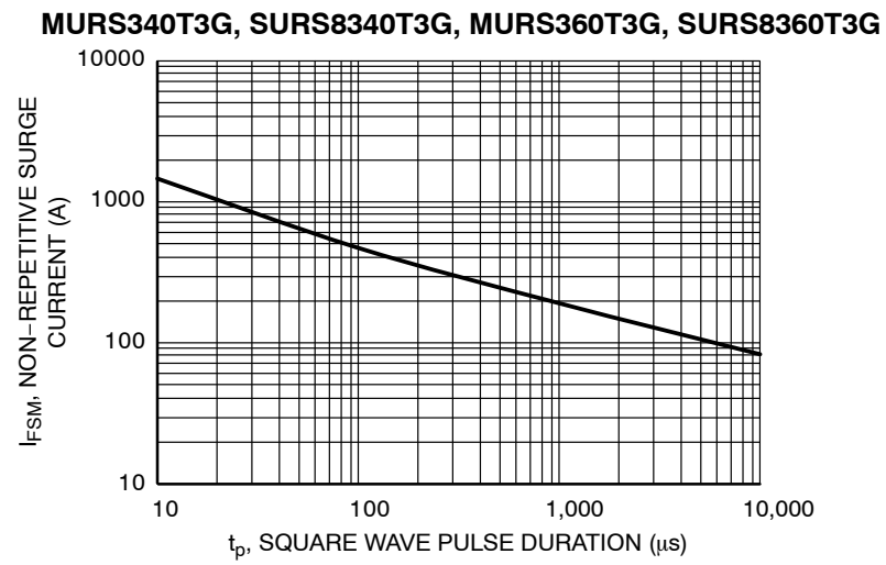
Figure 11. Typical Non-Repetitive Surge Current
