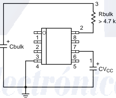
Figure 22. A simple resistor in series avoids any latchup in the controller
