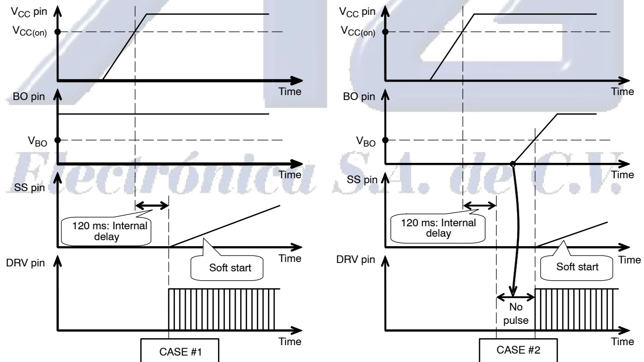
Figure 30. Different Startup Sequence Case #1 &amp; #2
