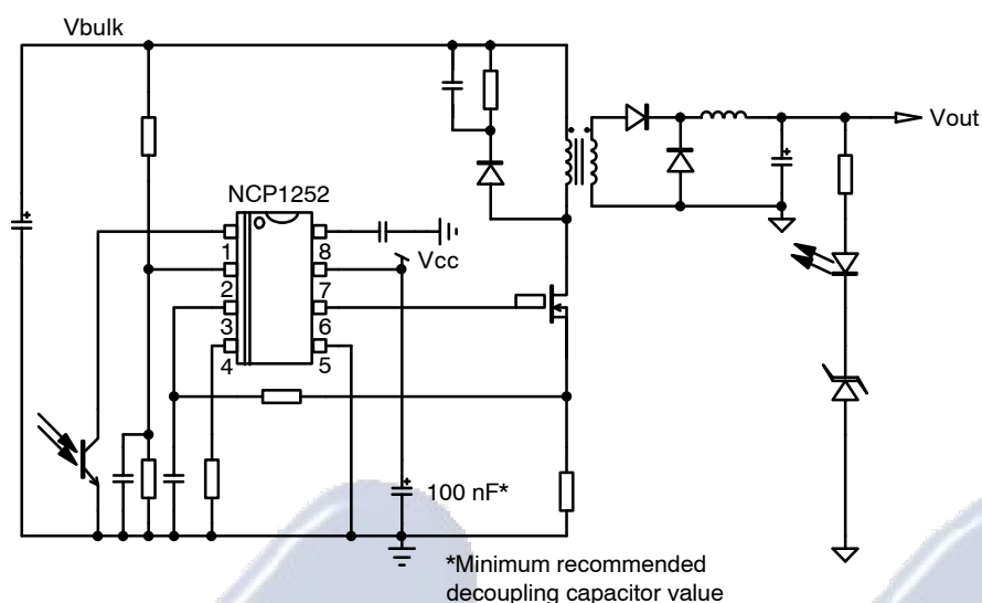
Figure 1. Typical Application
