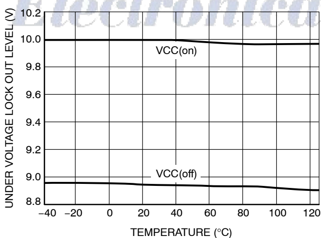
Figure 3. Supply Voltage Threshold vs. Junction Temperature
