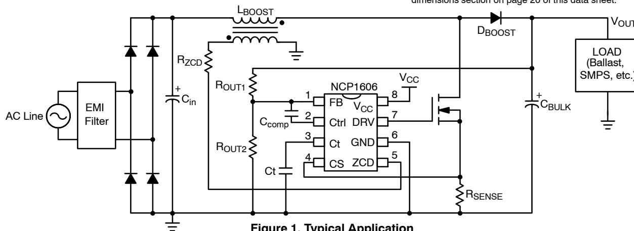
Figure 1. Typical Application
