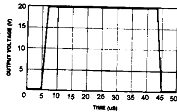
Figure 6. Slew Rate
