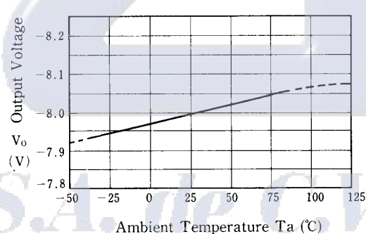
NJM79L08 Output Voltage vs. Temperature
