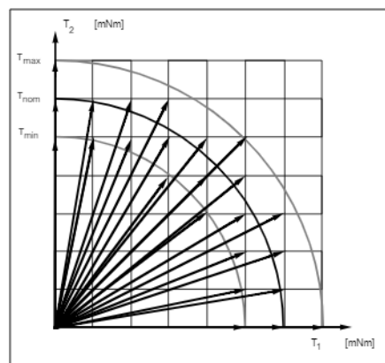
Figure 6b. An example of accessible positions with a given torque deviation/fullstep. Note that 1:st step sets highest resolution. Data points are exaggerated for illustration purpose.
