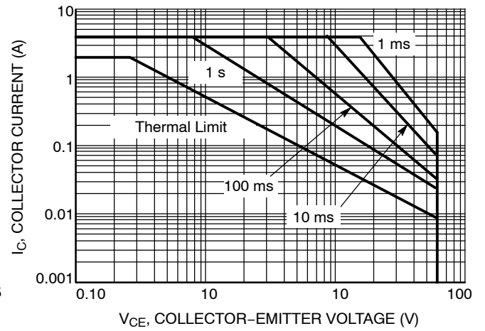
Figure 8. Safe Operating Area Single Pulse Test @ T_{amb} = 25^\circ\text{C}
