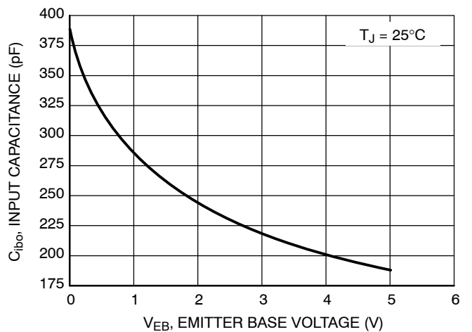
Figure 6. Input Capacitance
