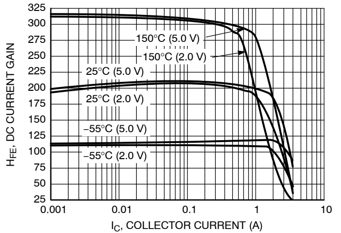
Figure 2. DC Current versus Collector Current
