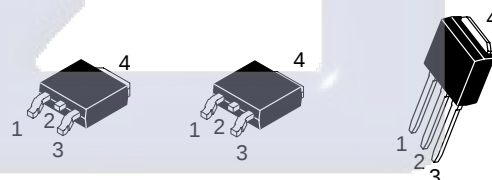
CASE 369AA DPAK (Surface Mount) STYLE 2
