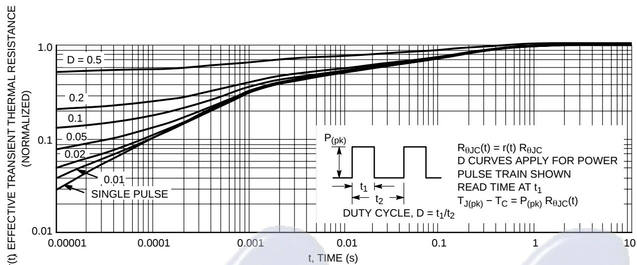
Figure 12. Thermal Response
