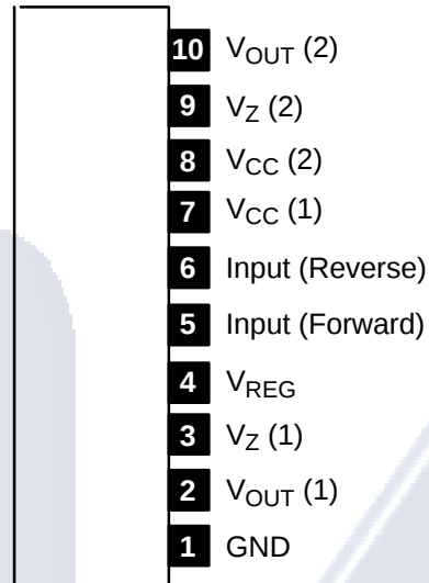
Pin Connection Diagram (Front View)
